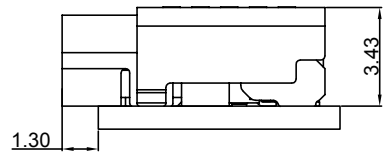
MOUNTING CONDITION(REF.)
